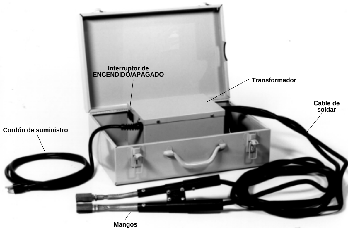
Figura 2a – Pistola de soldar RT-175
