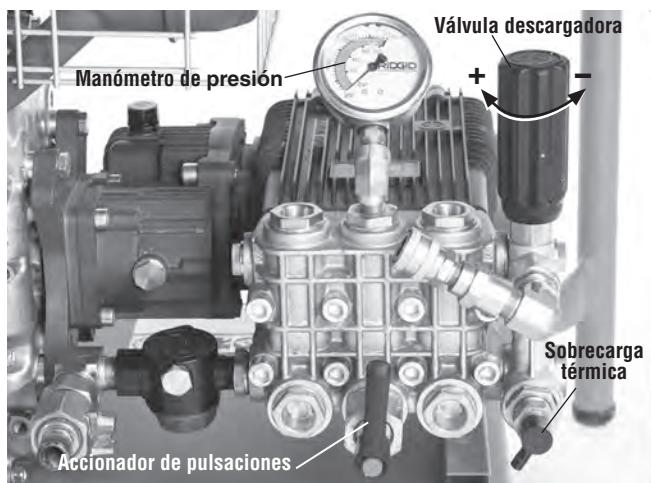
Figura 15 – Controles
