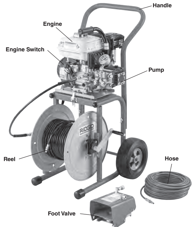
Figure 1 – KJ-2200 Water Jetting Machine
