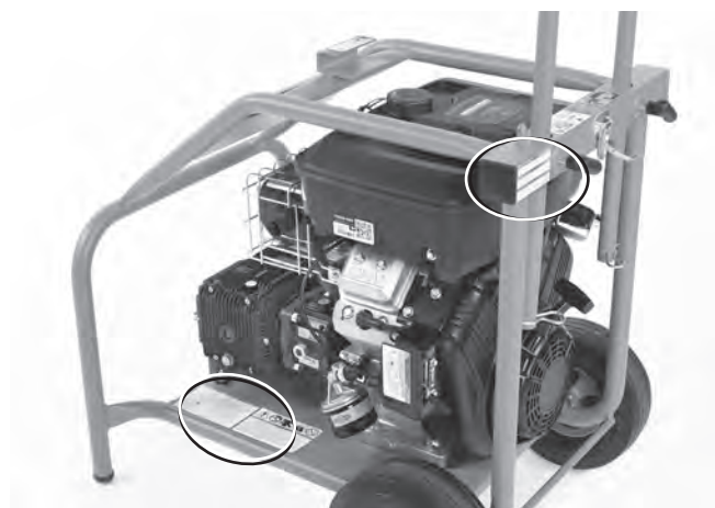
Figure 7F – KJ-3100 Warning Labels
