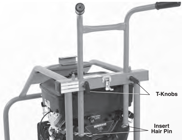
Figure 6 – KJ-3100 Handle Assembly
