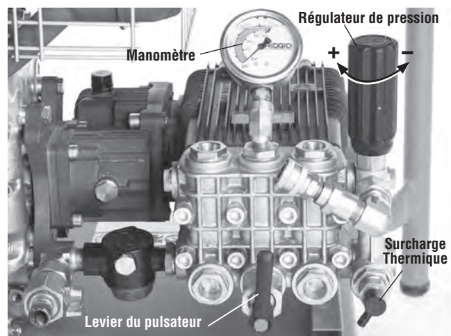
Figure 15 – Commandes
