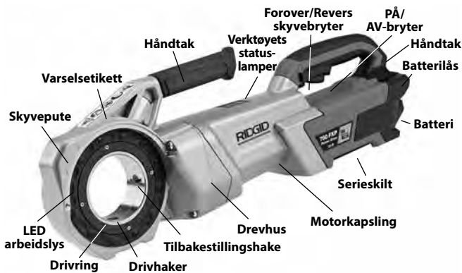
Figur 1 - 760 FXP Power Drive
