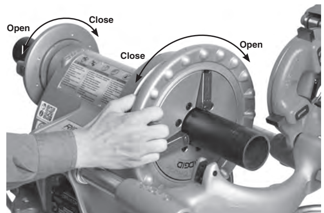
Figure 14 – Chucking Pipe
