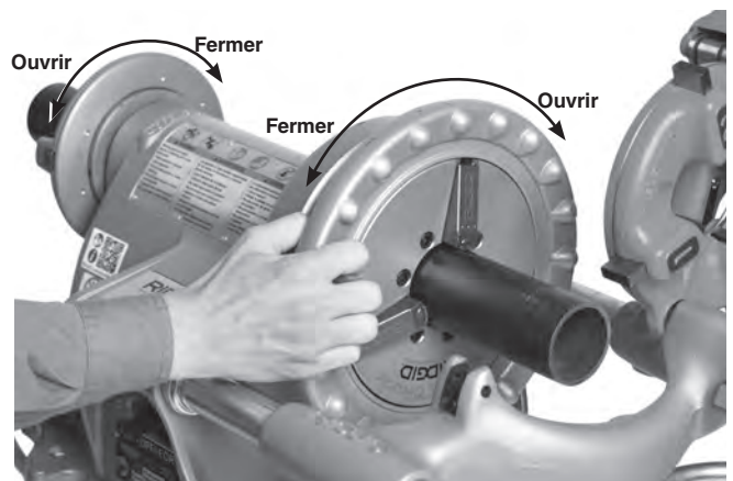
Figure 14 – Mandrinage du tuyau
