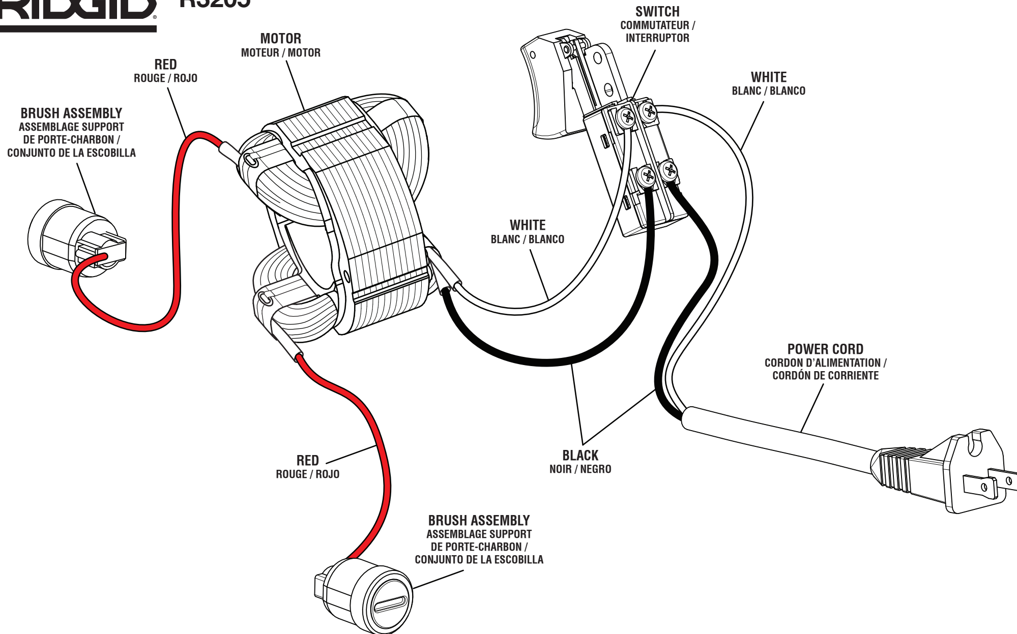
Wiring Diagram
