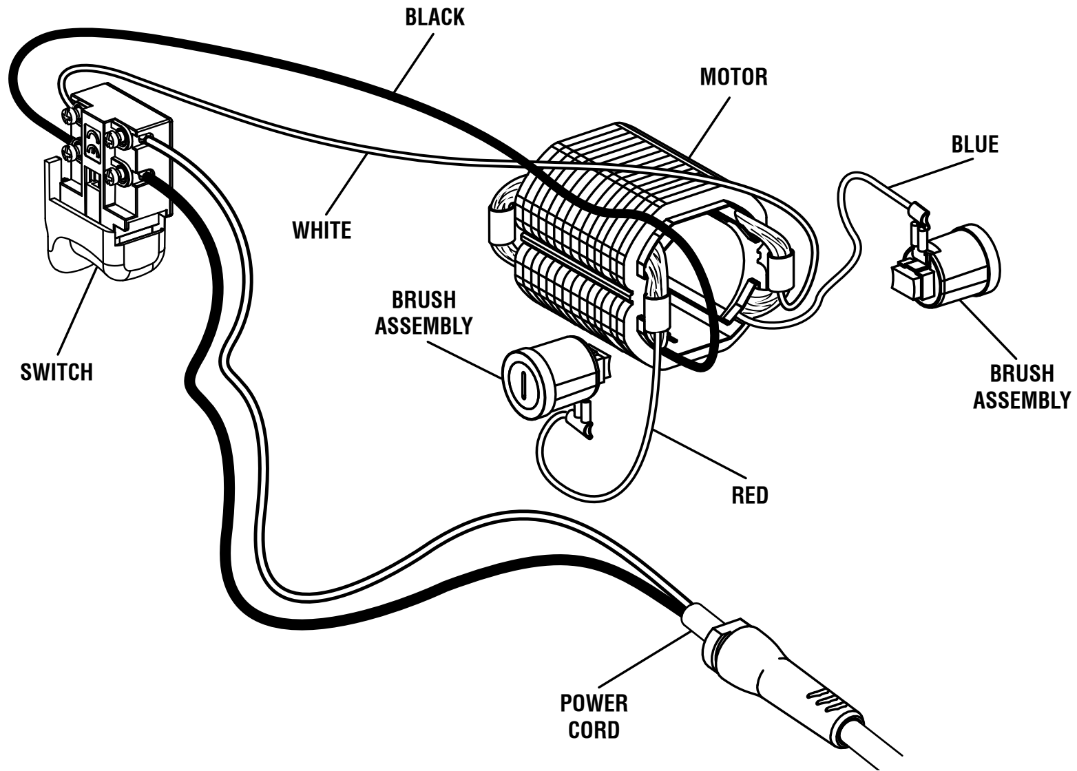
WIRING DIAGRAM
