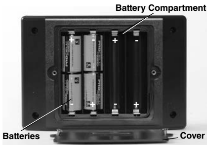
Figure 6 – Changing the Batteries (Transmitter)
