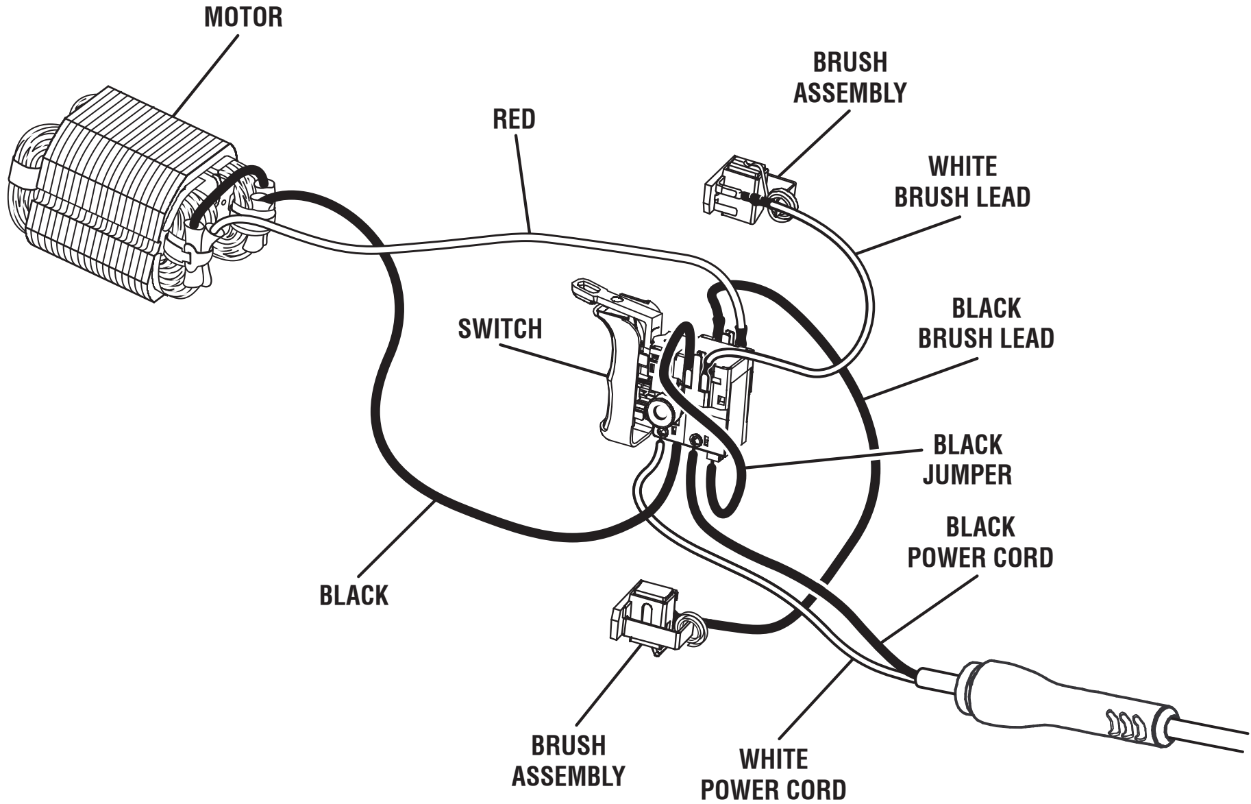
WIRING DIAGRAM
