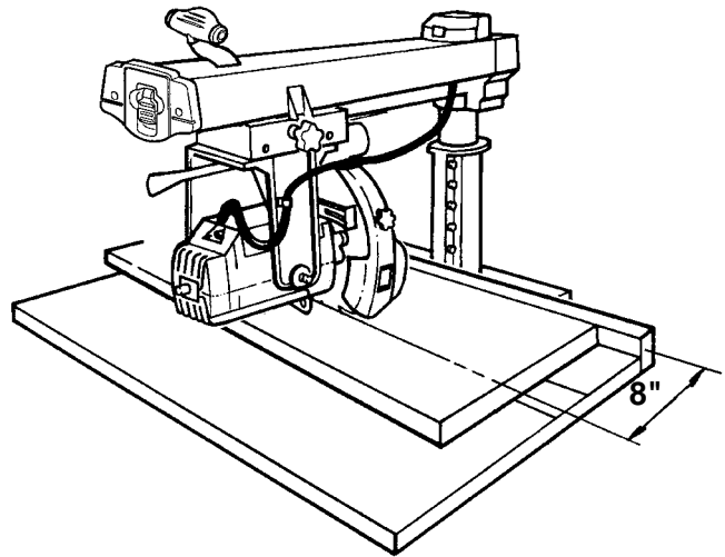
Example: To rip 2" off a 10" wide board, set blade in in-rip position 8" from rear fence.
