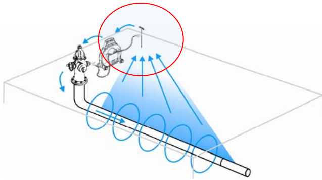
From the transmitter, down the line, back through the dirt it then needs to complete the circuit to the transmitter.
